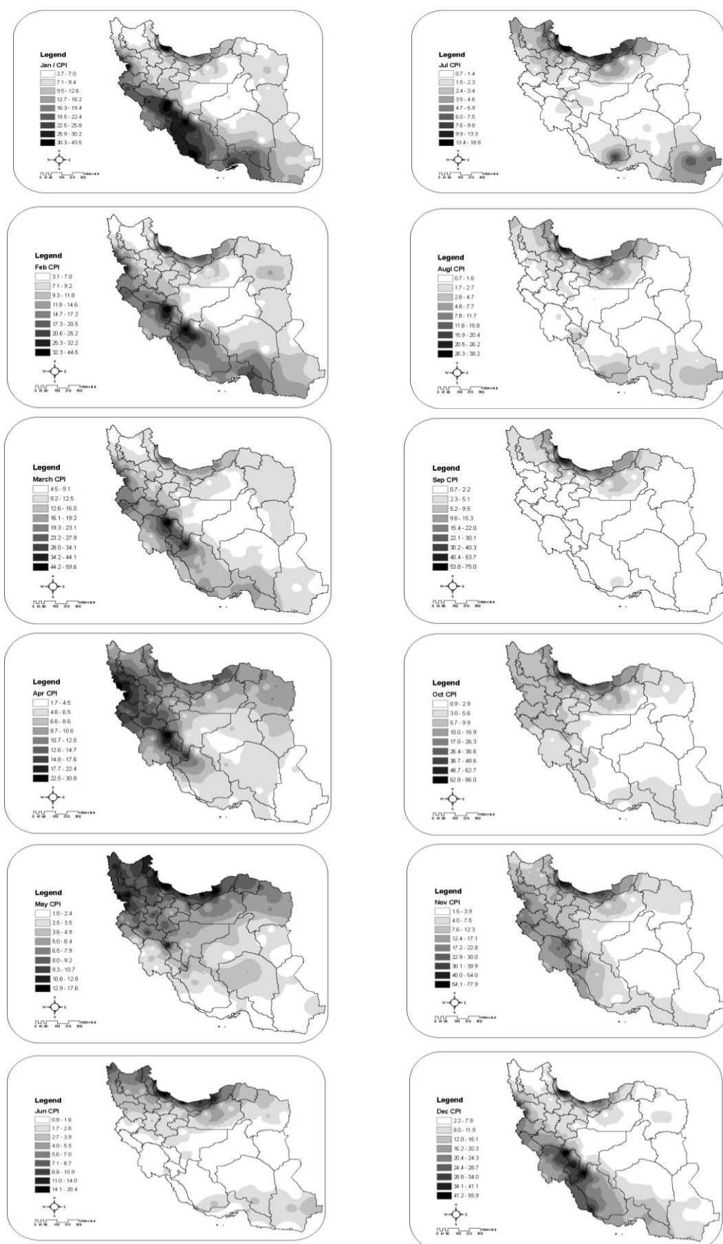
Fig. 3. Monthly CPI spatial distribution computation over Iran
